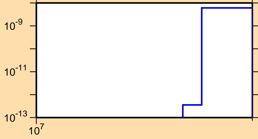
\sigma vs. E for ^{106}\text{Pd}(n,\text{nd})
