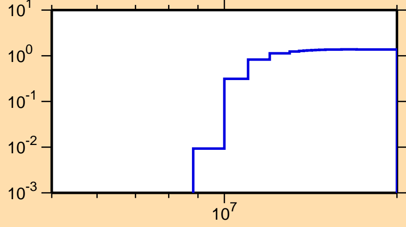
\sigma vs. E for ^{106}\text{Pd}(n,2n)
