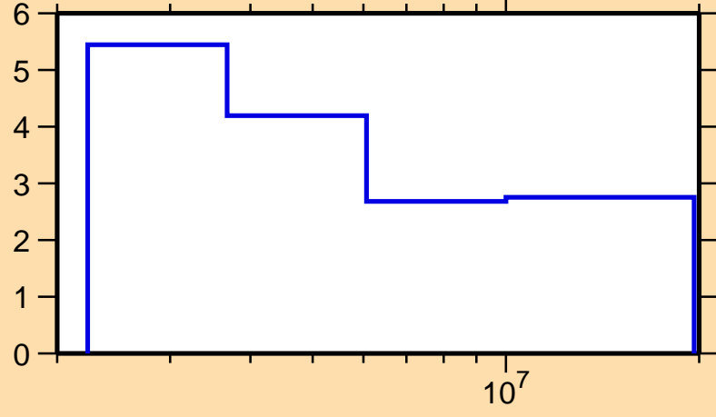
\Delta\sigma/\sigma vs. E for ^{106}\text{Pd}(n,n\text{nonel.})
