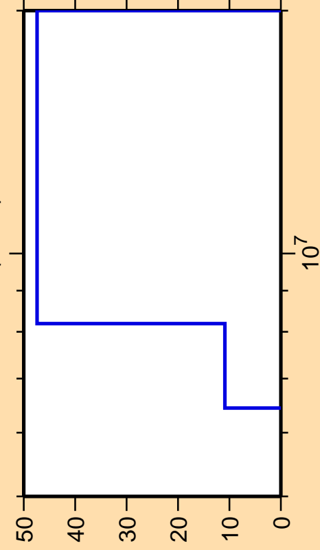
\Delta\sigma/\sigma vs. E for ^{106}\text{Pd}(n,n\alpha)
