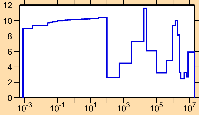
\Delta\sigma/\sigma vs. E for ^{106}\text{Pd}(n,\text{tot.})
