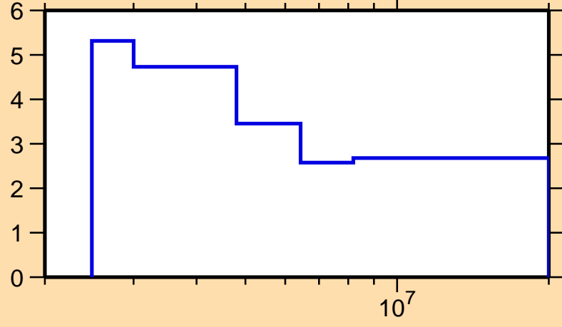
\Delta\sigma/\sigma vs. E for ^{106}\text{Pd}(n,\text{nonel.})
