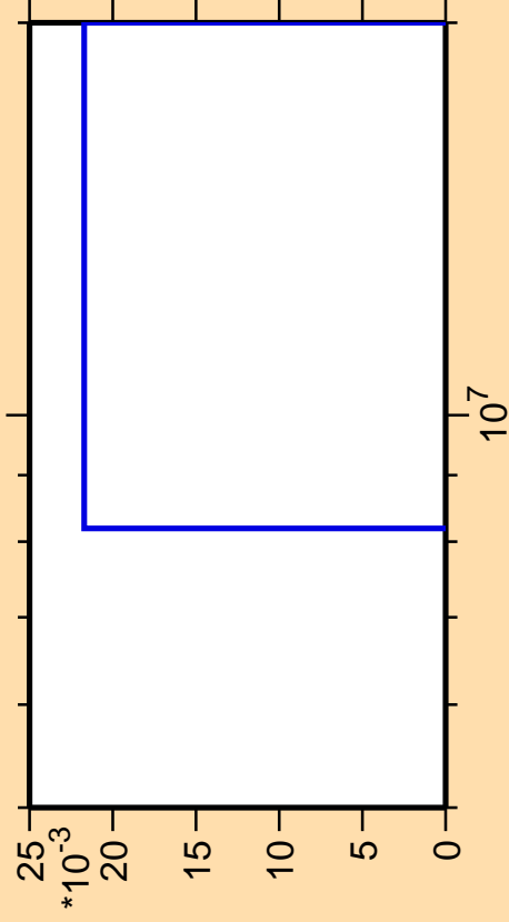
\Delta\sigma/\sigma vs. E for ^{106}\text{Pd}(n,p\alpha)
