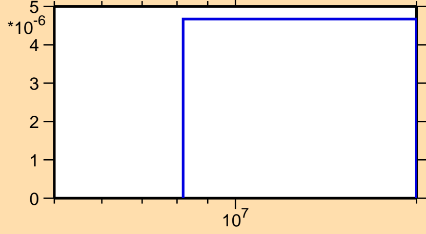
\sigma vs. E for ^{106}\text{Pd}(n,t)
