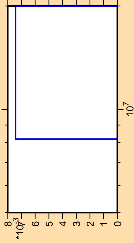
\Delta\sigma/\sigma vs. E for ^{106}\text{Pd}(n,2np)
