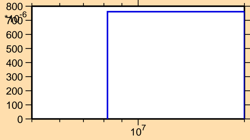
\sigma vs. E for ^{106}\text{Pd}(n,d)
