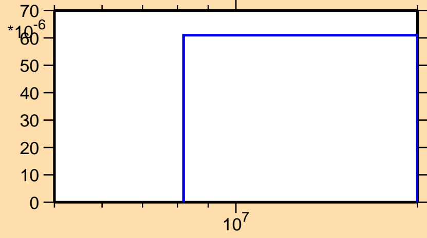
\sigma vs. E for ^{106}\text{Pd}(n,3n)
