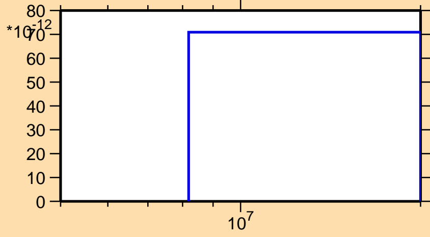
\sigma vs. E for ^{106}\text{Pd}(n,\text{He3})
