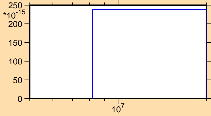
\sigma vs. E for ^{106}\text{Pd}(n,nt)
