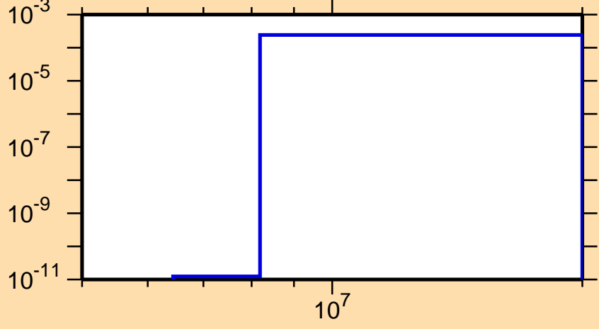
\sigma vs. E for ^{106}\text{Pd}(n,n\alpha)
