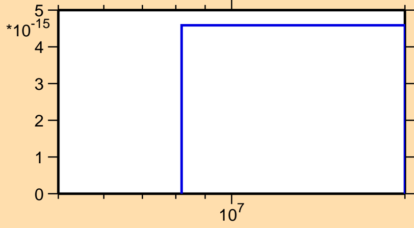
\sigma vs. E for ^{106}\text{Pd}(n,2np)
