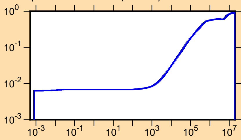
\mu vs. E for ^{107}\text{Pd}(\text{mt251})
