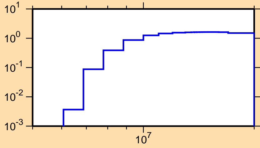
\sigma vs. E for ^{107}\text{Pd}(n,2n)
