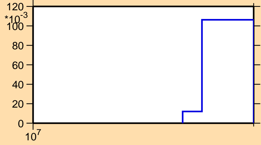
\sigma vs. E for ^{107}\text{Pd}(n,3n)
