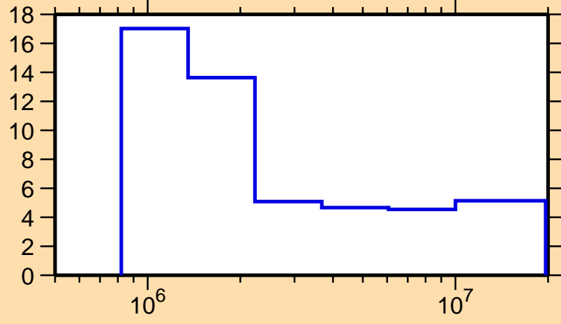
\Delta\sigma/\sigma vs. E for ^{107}\text{Pd}(n,n\text{onel.})
