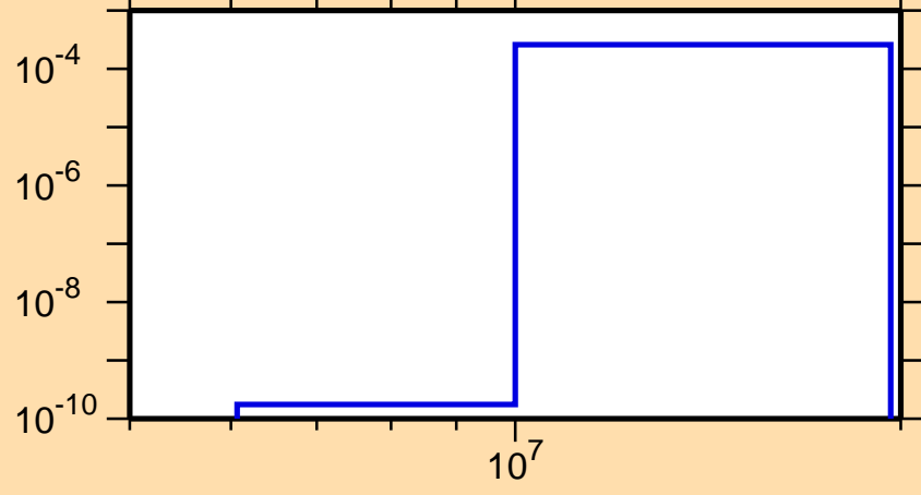
\sigma vs. E for ^{107}\text{Pd}(n,n\alpha)
