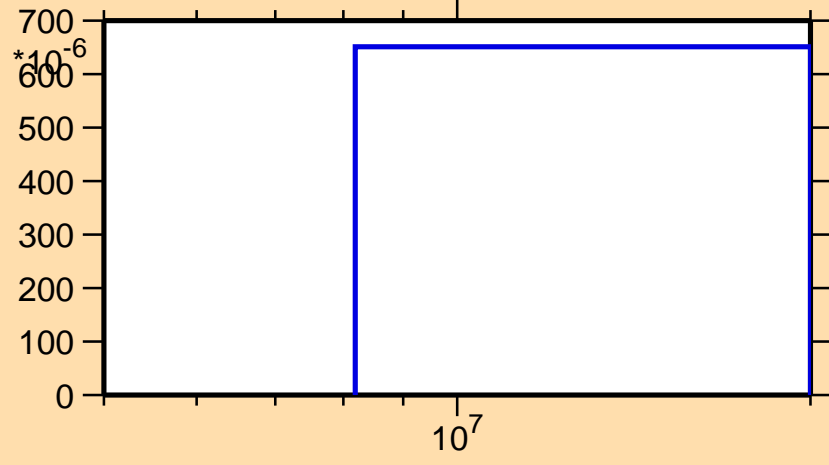
\sigma vs. E for ^{107}\text{Pd}(n,np)
