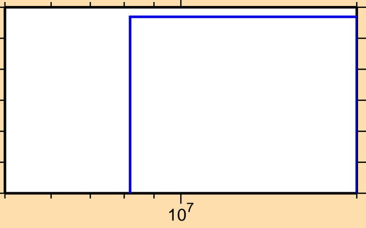
\sigma vs. E for ^{107}\text{Pd}(n,d)
