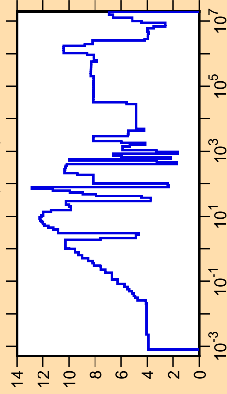
\Delta\sigma/\sigma vs. E for ^{108}\text{Pd}(n,\text{tot.})
