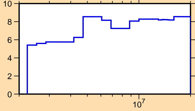
\Delta\sigma/\sigma vs. E for ^{108}\text{Pd}(n,n\text{onel.})
