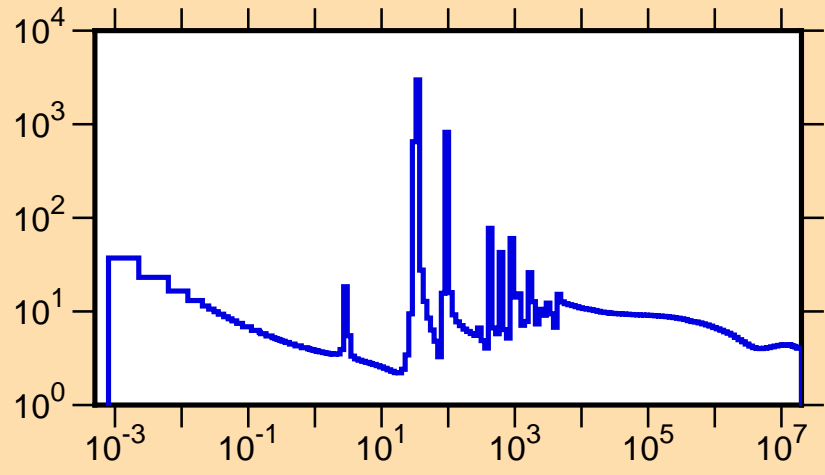
\sigma vs. E for ^{108}\text{Pd}(n,\text{tot.})
