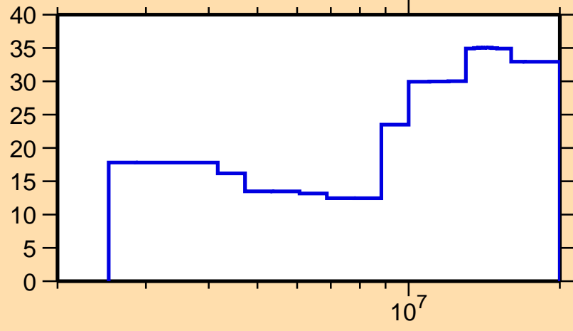
\Delta\sigma/\sigma vs. E for ^{108}\text{Pd}(n,n\text{cont.})
