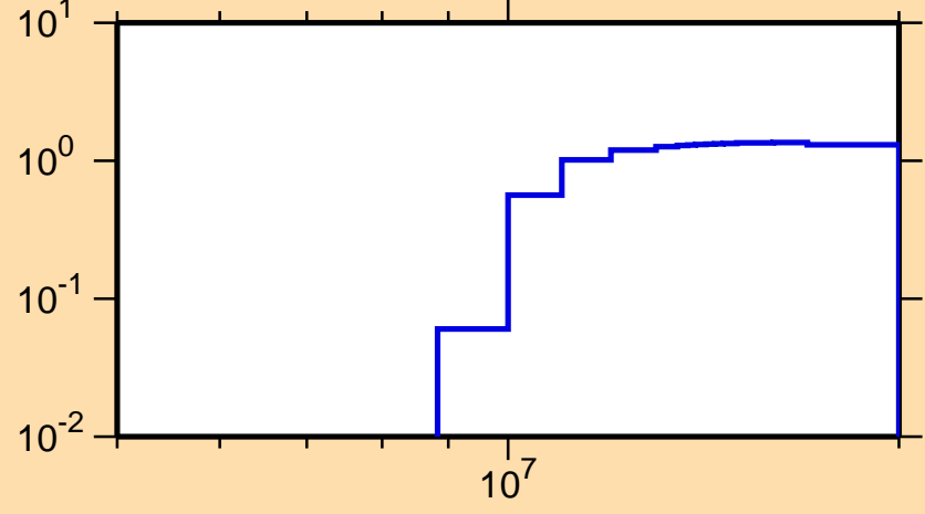
\sigma vs. E for ^{108}\text{Pd}(n,2n)
