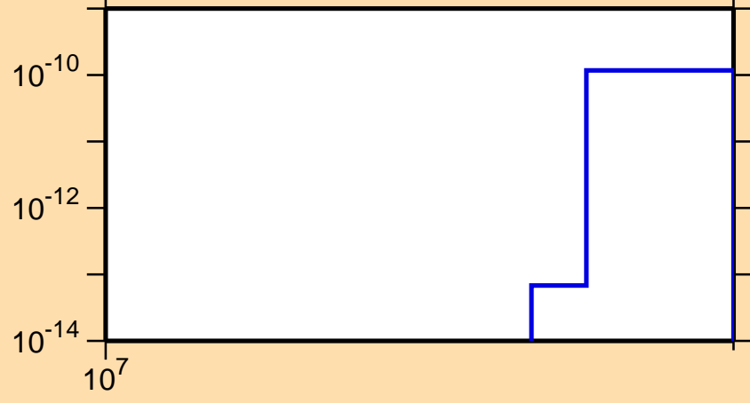
\sigma vs. E for ^{108}\text{Pd}(n,\text{He}3)
