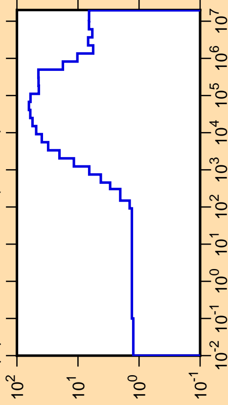
\Delta\mu/\mu vs. E for ^{108}\text{Pd}(\text{mt251})
