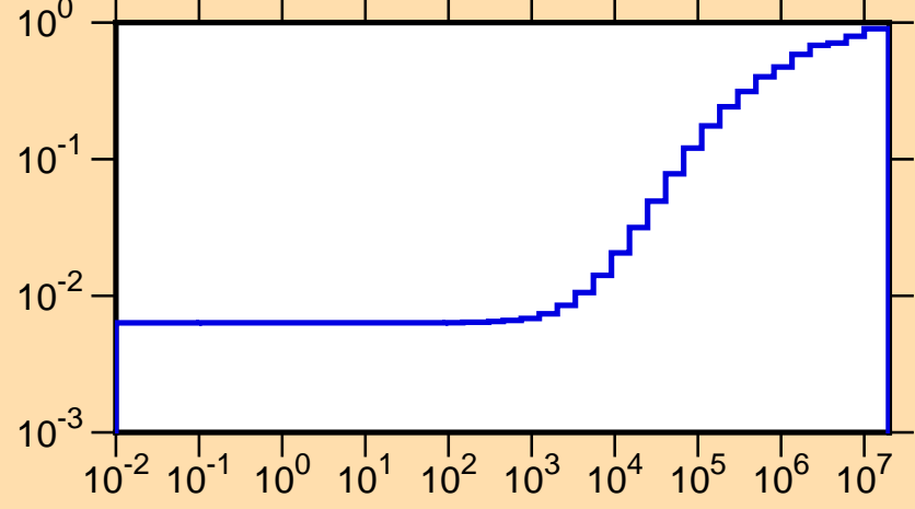
\mu vs. E for ^{108}\text{Pd}(\text{mt251})
