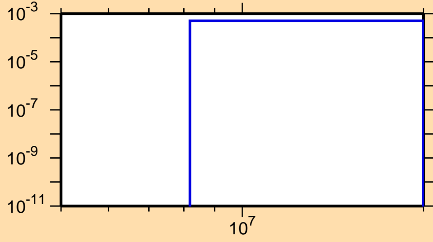
\sigma vs. E for ^{108}\text{Pd}(n,d)
