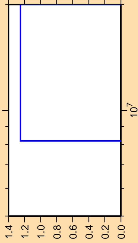
\Delta\sigma/\sigma vs. E for ^{108}\text{Pd}(n,\text{nt})
