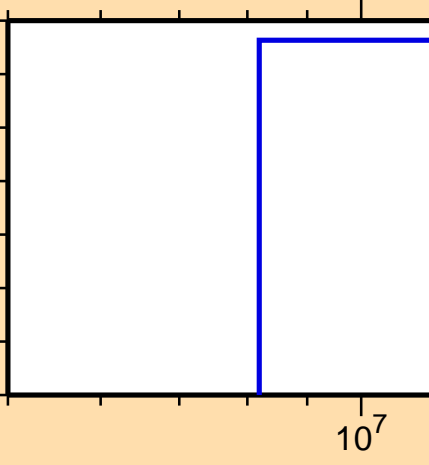
\sigma vs. E for ^{108}\text{Pd}(n,\text{nd})
