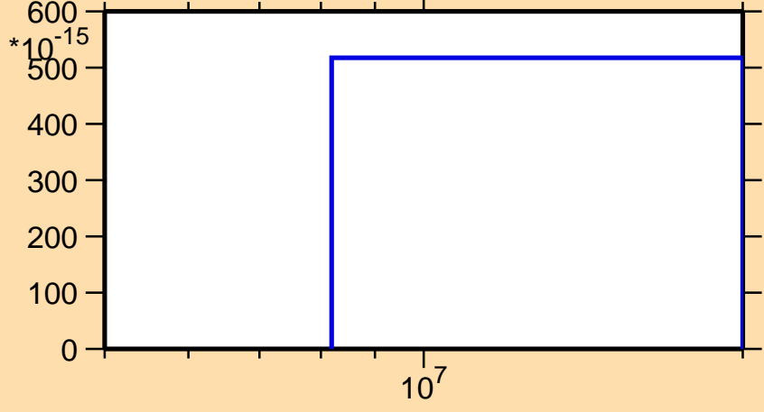
\sigma vs. E for ^{108}\text{Pd}(n,\text{nt})
