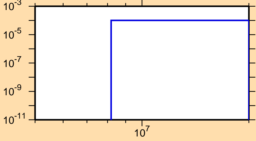
\sigma vs. E for ^{108}\text{Pd}(n,n\alpha)
