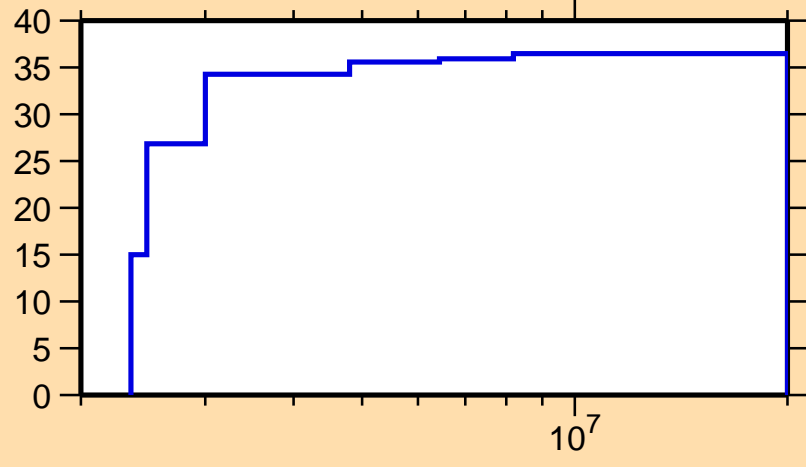
\Delta\sigma/\sigma vs. E for ^{108}\text{Pd}(n,n_1)
