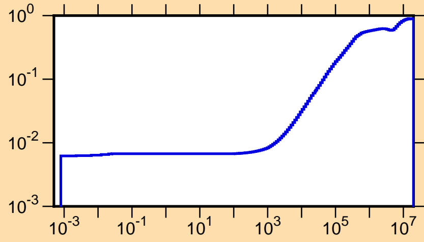
\mu vs. E for ^{109}\text{Pd}(\text{mt251})
