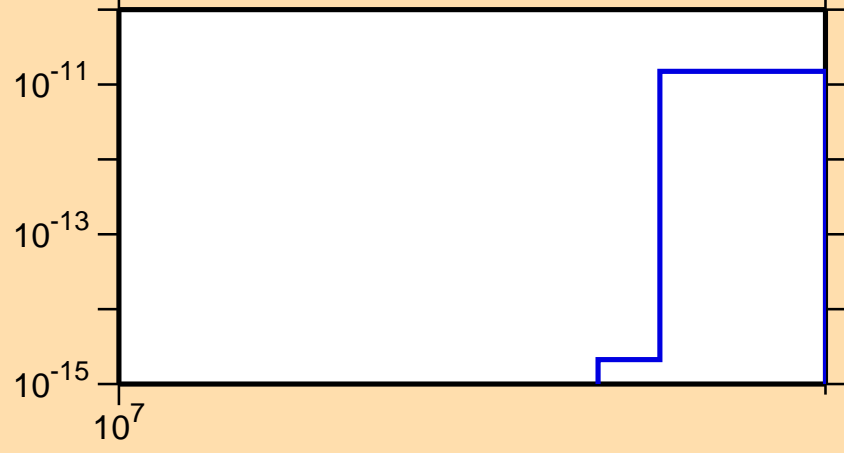
\sigma vs. E for ^{109}\text{Pd}(n,\text{He}3)
