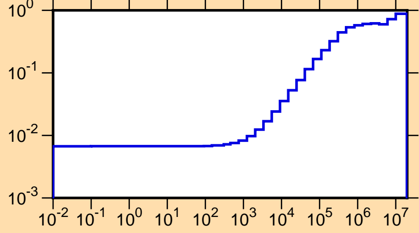
\mu vs. E for ^{109}\text{Pd}(\text{mt251})
