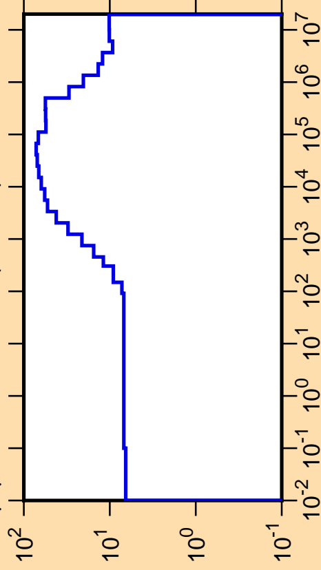
\Delta\mu/\mu vs. E for ^{109}\text{Pd}(\text{mt251})
