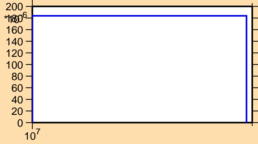
\sigma vs. E for ^{109}\text{Pd}(n,np)
