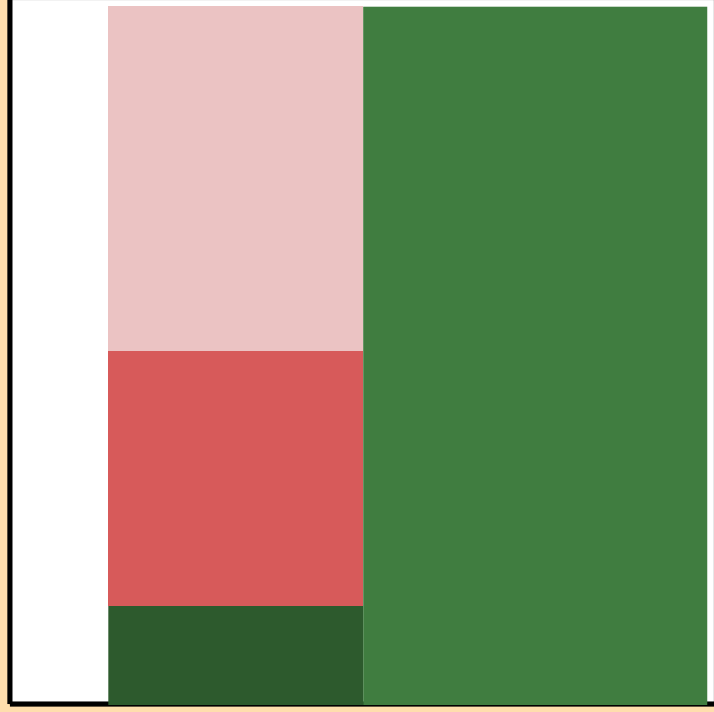
\Delta\sigma/\sigma vs. E for ^{109}\text{Pd}(n,2n)
