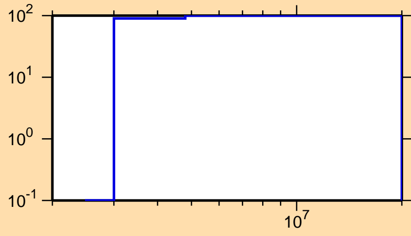
\Delta\sigma/\sigma vs. E for ^{109}\text{Pd}(n,p)
