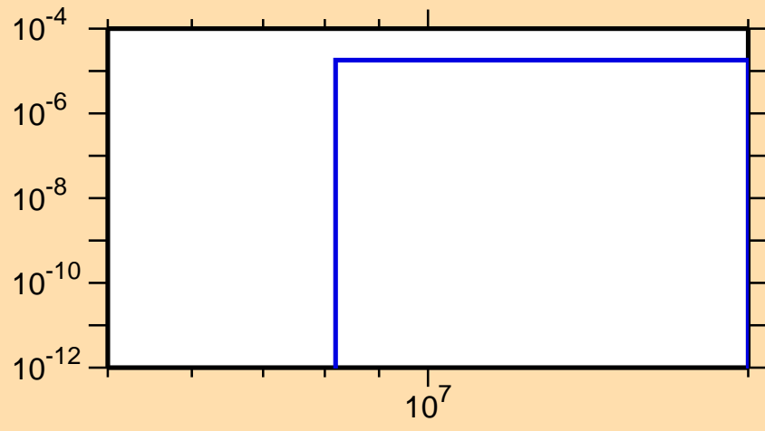
\sigma vs. E for ^{109}\text{Pd}(n,t)
