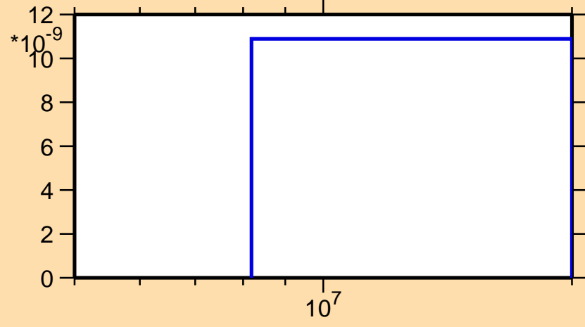
\sigma vs. E for ^{109}\text{Pd}(n,\text{nd})
