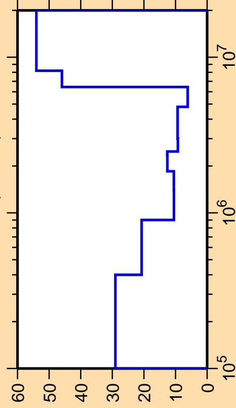
\Delta\sigma/\sigma vs. E for ^{109}\text{Pd}(n,\text{inel.})
