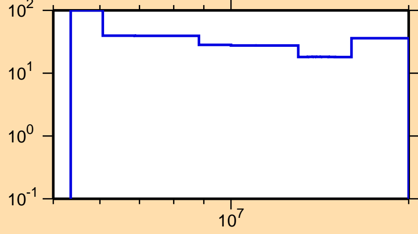
\Delta\sigma/\sigma vs. E for ^{109}\text{Pd}(n,2n)
