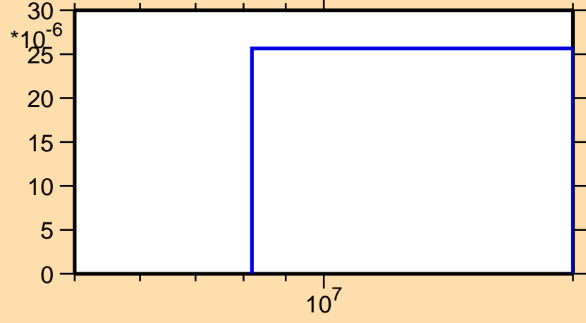
\sigma vs. E for ^{109}\text{Pd}(n,t)
