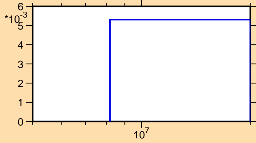
\sigma vs. E for ^{109}\text{Pd}(n,3n)
