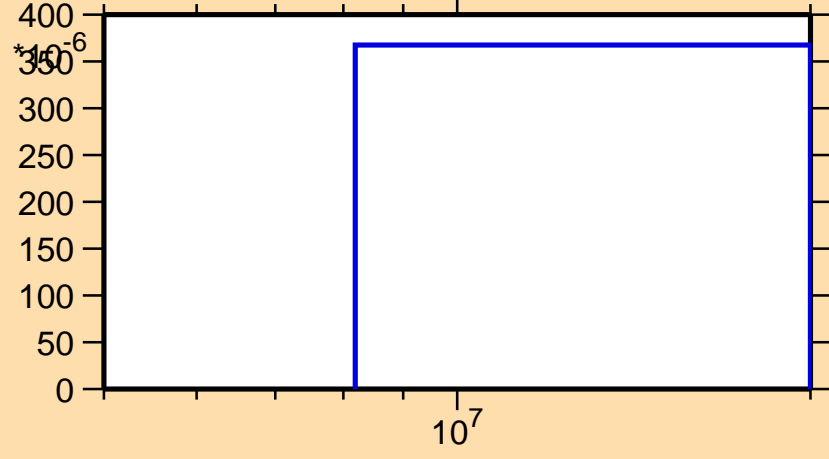
\sigma vs. E for ^{109}\text{Pd}(n,d)
