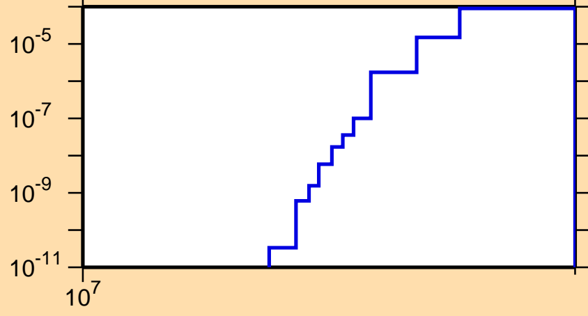
\sigma vs. E for ^{110}\text{Pd}(n,t)
