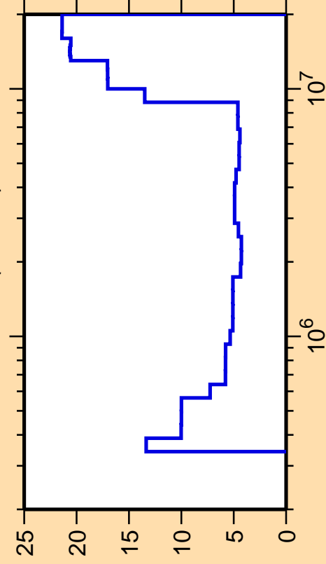
\Delta\sigma/\sigma vs. E for ^{110}\text{Pd}(n,\text{inel.})
