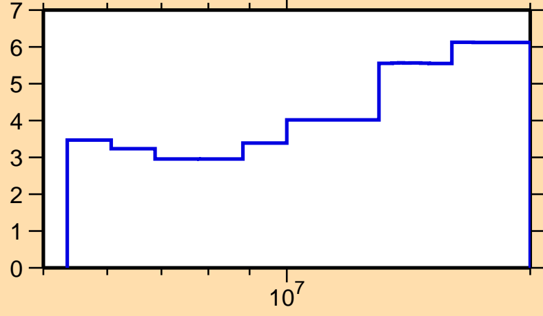
\Delta\sigma/\sigma vs. E for ^{110}\text{Pd}(n,\text{tot.})
