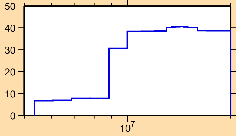
\Delta\sigma/\sigma vs. E for ^{110}\text{Pd}(n,ncont.)
