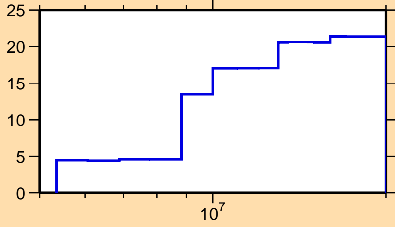
\Delta\sigma/\sigma vs. E for ^{110}\text{Pd}(n,\text{inel.})
