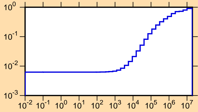
\mu vs. E for ^{110}\text{Pd}(\text{mt251})
