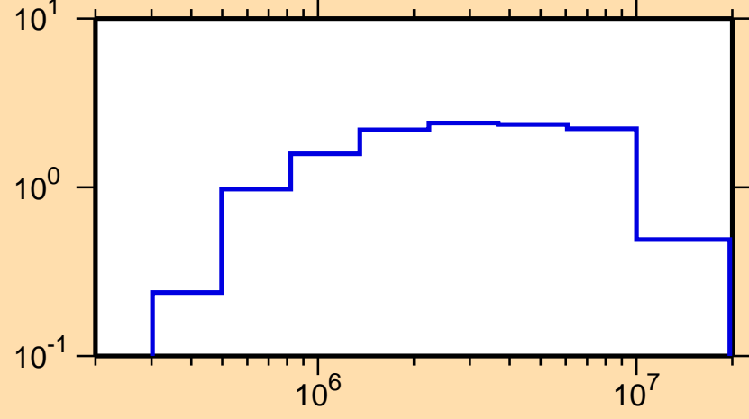
\sigma vs. E for ^{110}\text{Pd}(n,\text{inel.})
