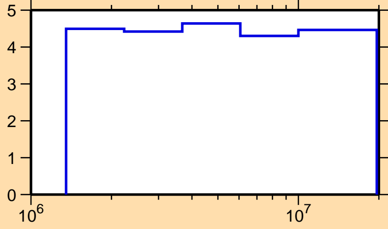
\Delta\sigma/\sigma vs. E for ^{110}\text{Pd}(n,n\text{nonel.})
