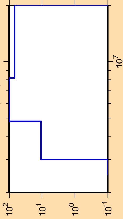
\Delta\sigma/\sigma vs. E for ^{110}\text{Pd}(n,\alpha)
