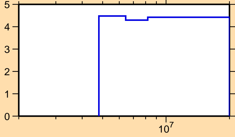
\Delta\sigma/\sigma vs. E for ^{110}\text{Pd}(n,\text{nonel.})
