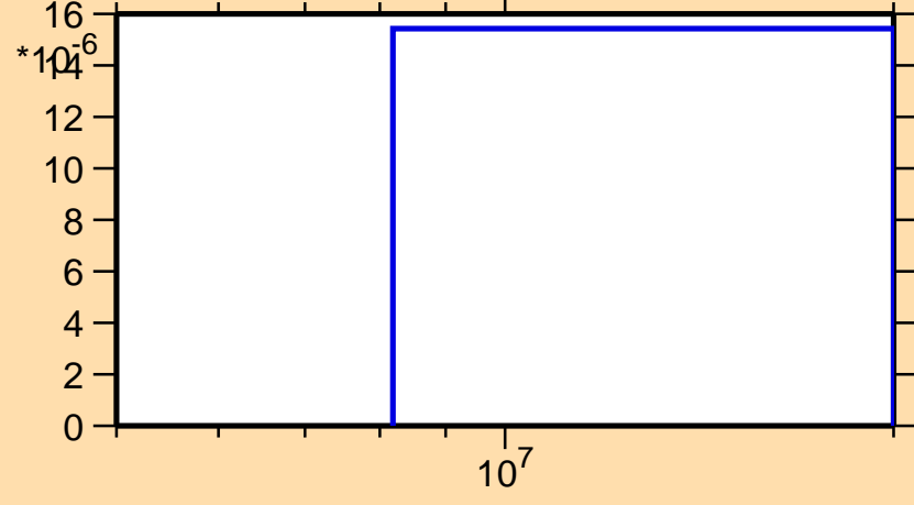
\sigma vs. E for ^{110}\text{Pd}(n,np)
