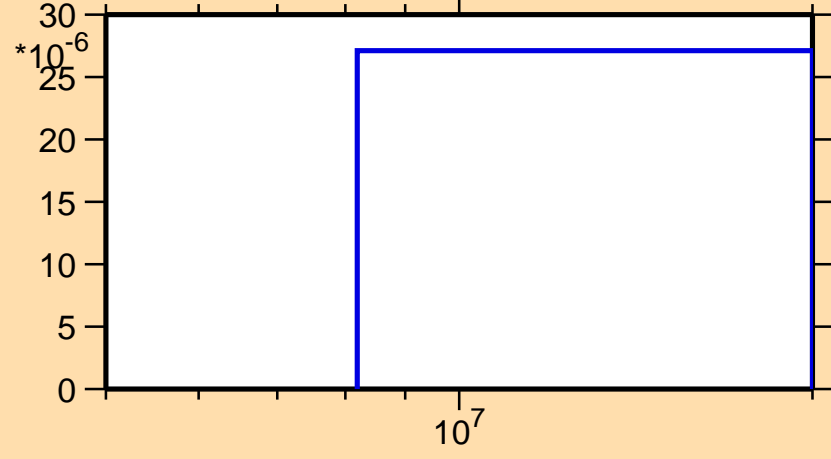
\sigma vs. E for ^{110}\text{Pd}(n,n\alpha)
