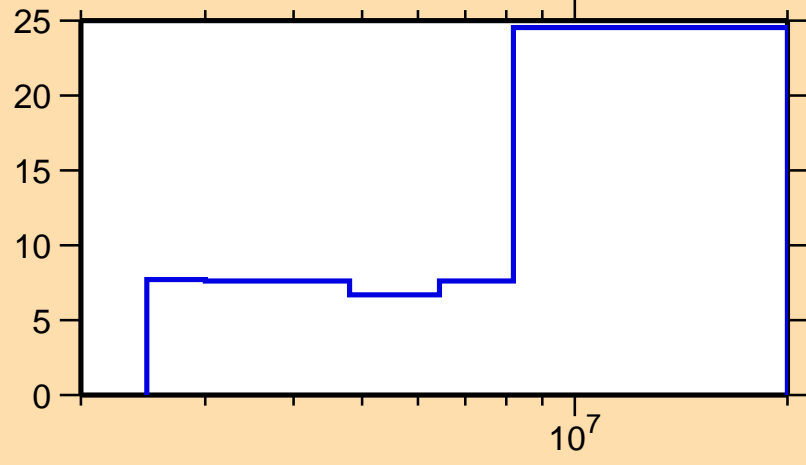
\Delta\sigma/\sigma vs. E for ^{110}\text{Pd}(n,n\text{cont.})
