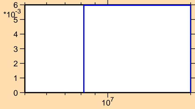
\sigma vs. E for ^{110}\text{Pd}(n,3n)
