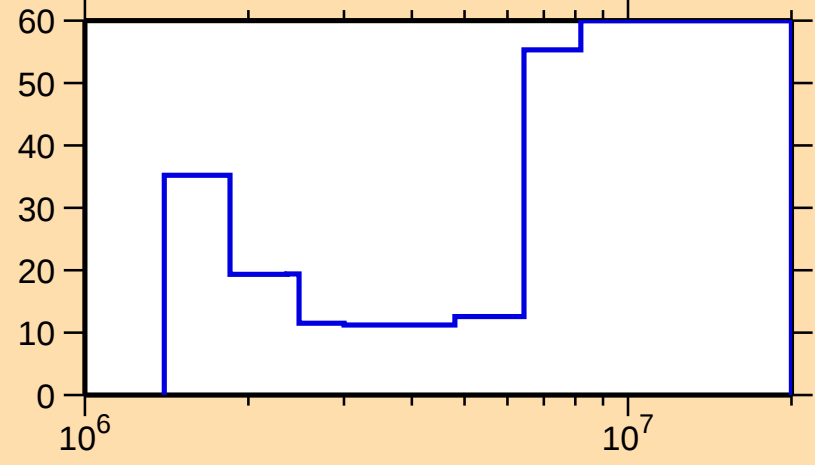
\Delta\sigma/\sigma vs. E for ^{111}\text{Pd}(n,n\text{cont.})
