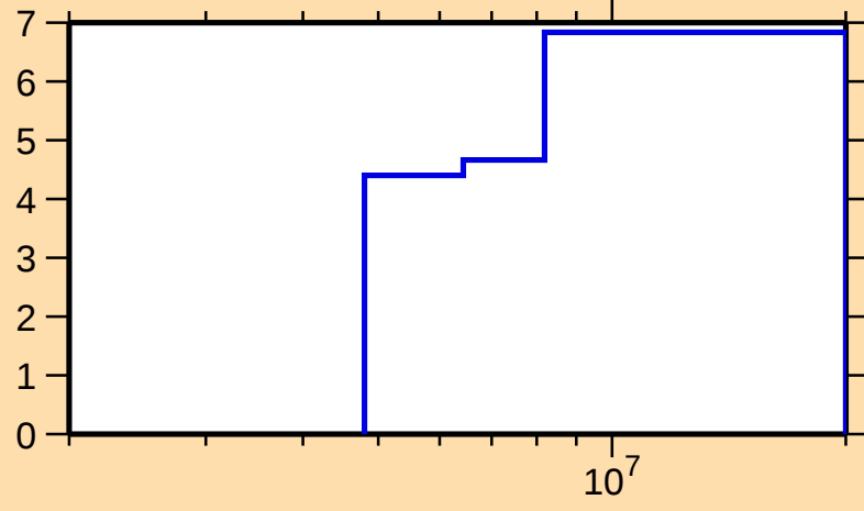
\Delta\sigma/\sigma vs. E for ^{111}\text{Pd}(n,\text{tot.})
