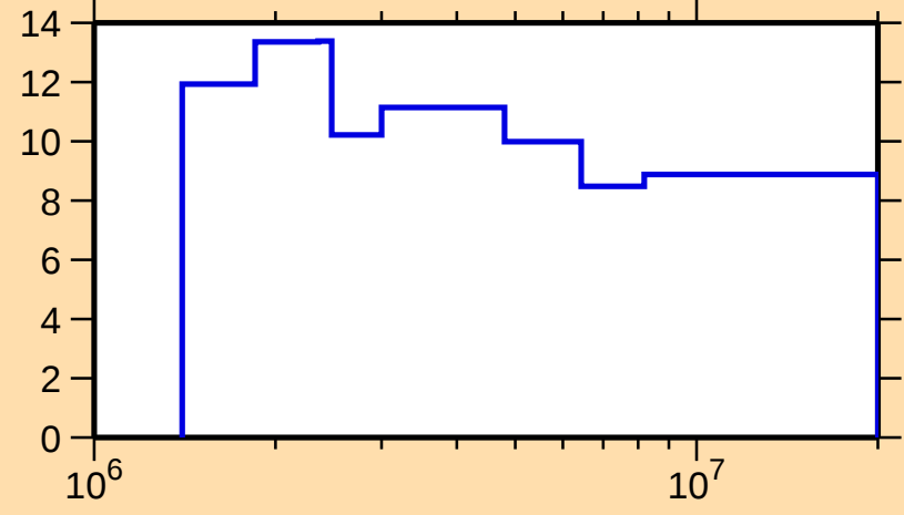
\Delta\sigma/\sigma vs. E for ^{111}\text{Pd}(n,\text{nonel.})
