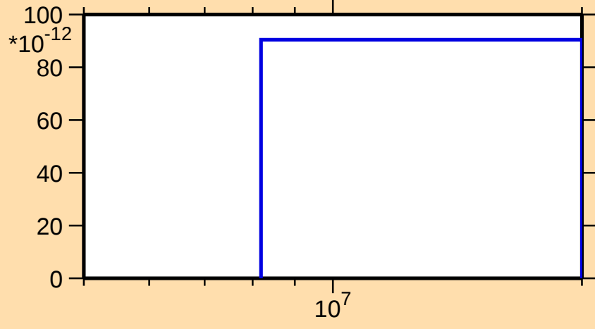
\sigma vs. E for ^{111}\text{Pd}(n,2np)
