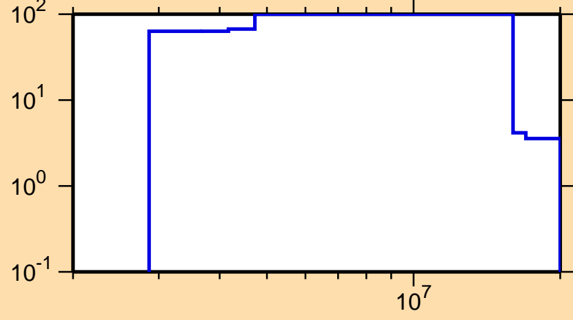
\Delta\sigma/\sigma vs. E for ^{111}\text{Pd}(n,n_1)
