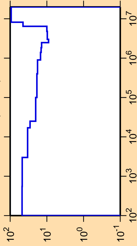
\Delta\sigma/\sigma vs. E for ^{111}\text{Pd}(n,\text{inel.})
