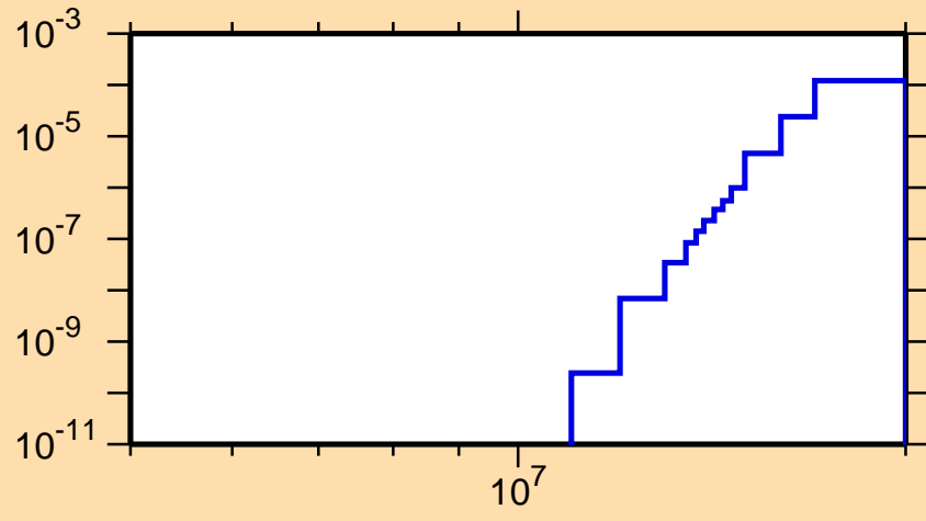
\sigma vs. E for ^{112}\text{Pd}(n,n\alpha)
