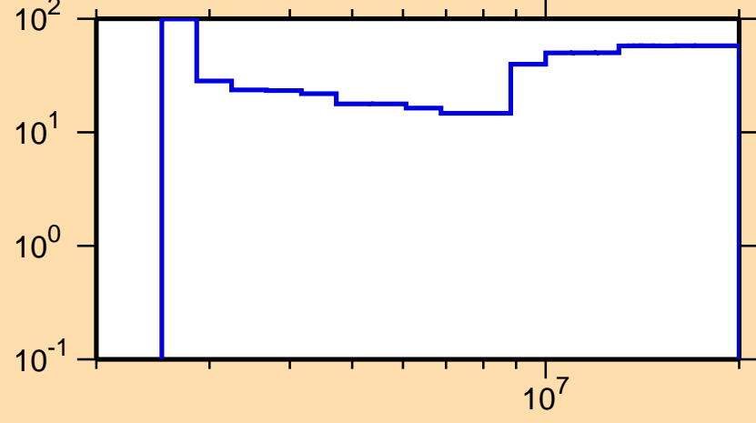
\Delta\sigma/\sigma vs. E for ^{112}\text{Pd}(n,n\text{cont.})
