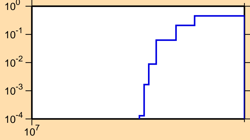
\sigma vs. E for ^{112}\text{Pd}(n,3n)
