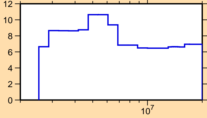
\Delta\sigma/\sigma vs. E for ^{112}\text{Pd}(n,n\text{inel.})
