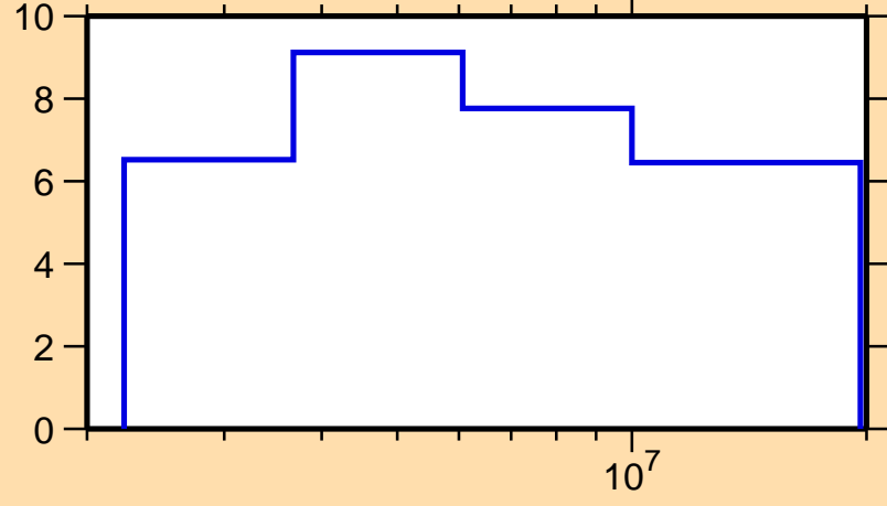
\Delta\sigma/\sigma vs. E for ^{112}\text{Pd}(n,n\text{nonel.})
