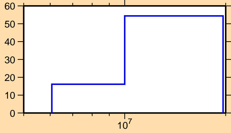
\Delta\sigma/\sigma vs. E for ^{112}\text{Pd}(n,ncont.)
