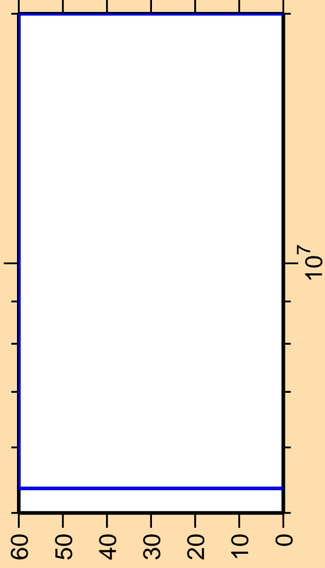
\Delta\sigma/\sigma vs. E for ^{113}\text{Pd}(n,\gamma)
