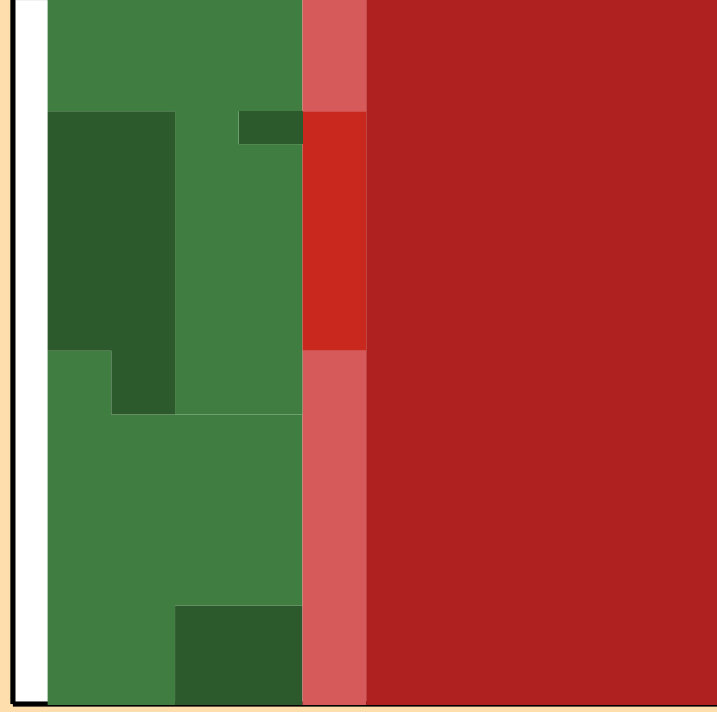
\Delta\sigma/\sigma vs. E for ^{113}\text{Pd}(n,2n)
