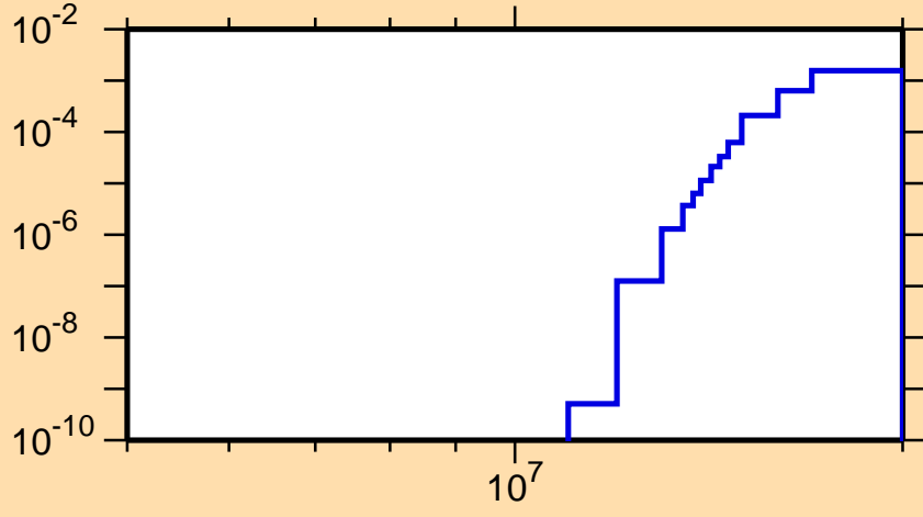
\sigma vs. E for ^{113}\text{Pd}(n,d)
