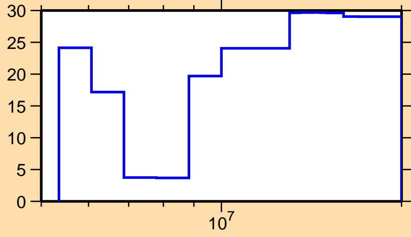
\Delta\sigma/\sigma vs. E for ^{113}\text{Pd}(n,\text{el.})
