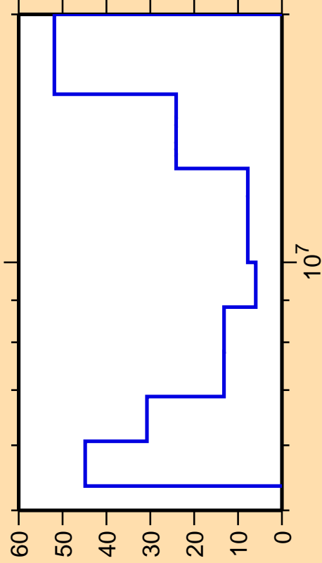
\Delta\sigma/\sigma vs. E for ^{113}\text{Pd}(n,2n)
