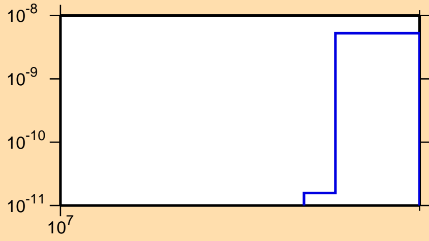
\sigma vs. E for ^{113}\text{Pd}(n,2n\alpha)
