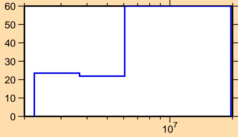
\Delta\sigma/\sigma vs. E for ^{113}\text{Pd}(n,n\text{cont.})
