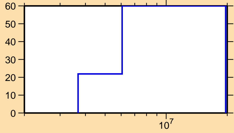
\Delta\sigma/\sigma vs. E for ^{113}\text{Pd}(n,ncont.)
