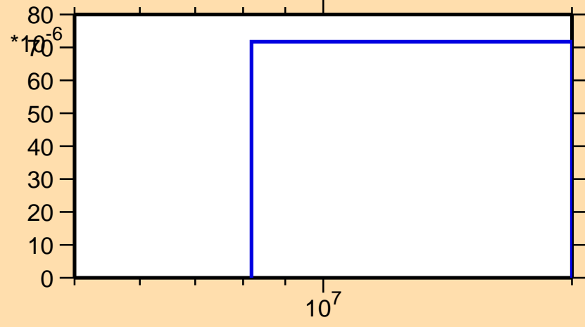
\sigma vs. E for ^{113}\text{Pd}(n,d)
