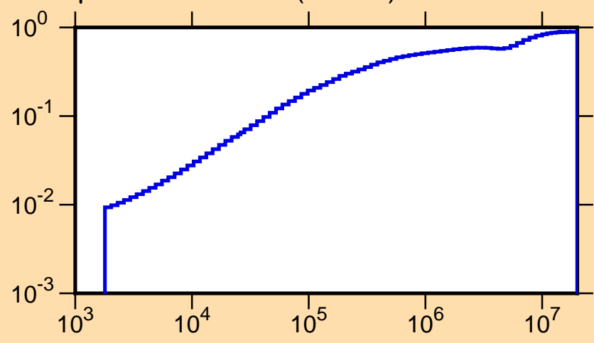
\mu vs. E for ^{114}\text{Pd}(\text{mt251})
