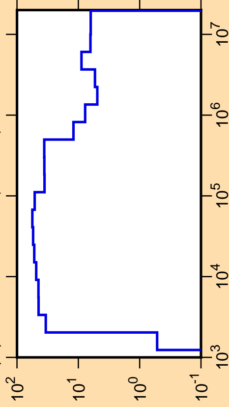
\Delta\mu/\mu vs. E for ^{114}\text{Pd}(\text{mt251})
