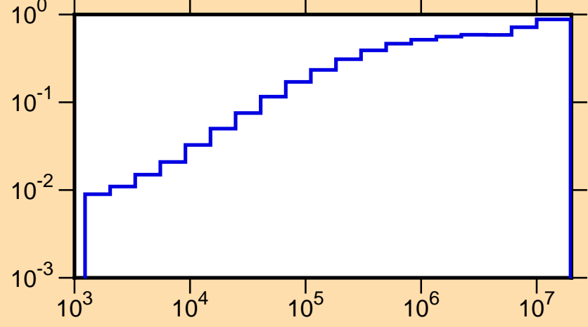
\mu vs. E for ^{114}\text{Pd}(\text{mt251})
