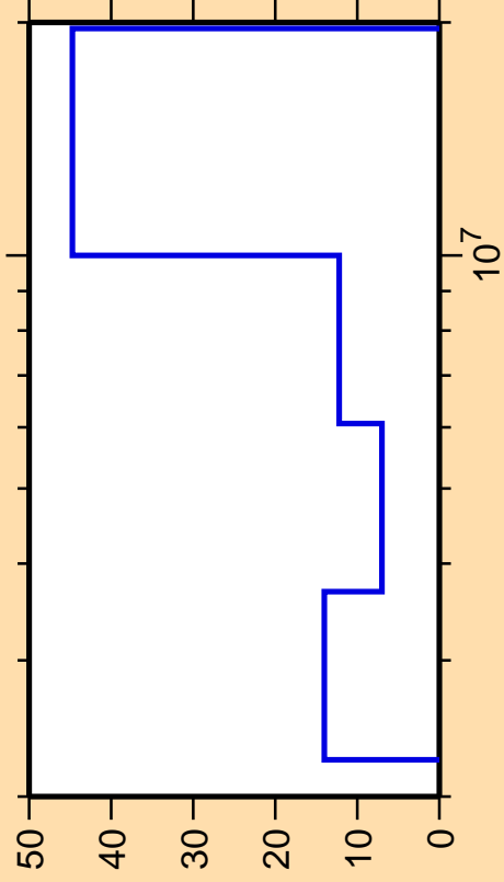
\Delta\sigma/\sigma vs. E for ^{114}\text{Pd}(n,\text{ncont.})
