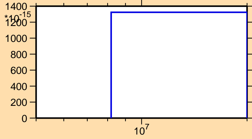
\sigma vs. E for ^{114}\text{Pd}(n,\text{nt})
