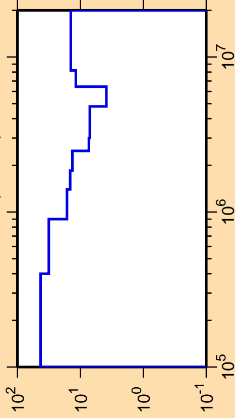
\Delta\sigma/\sigma vs. E for ^{114}\text{Pd}(n,\text{inel.})
