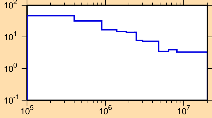
\Delta\sigma/\sigma vs. E for ^{114}\text{Pd}(n,\text{nonel.})
