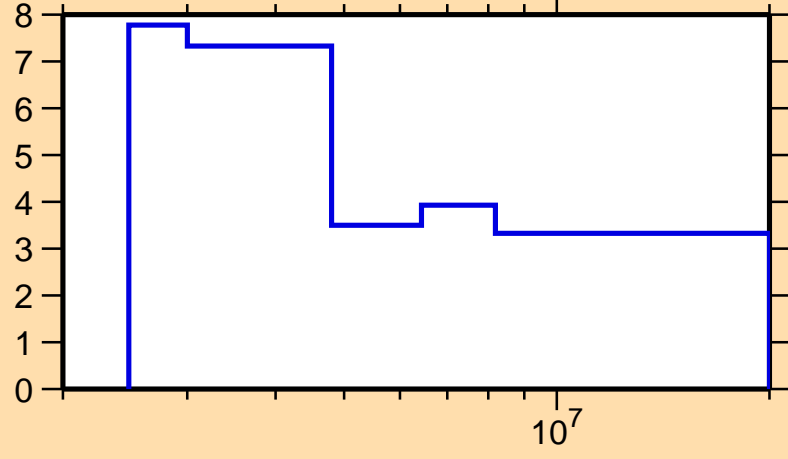
\Delta\sigma/\sigma vs. E for ^{114}\text{Pd}(n,n\text{nonel.})
