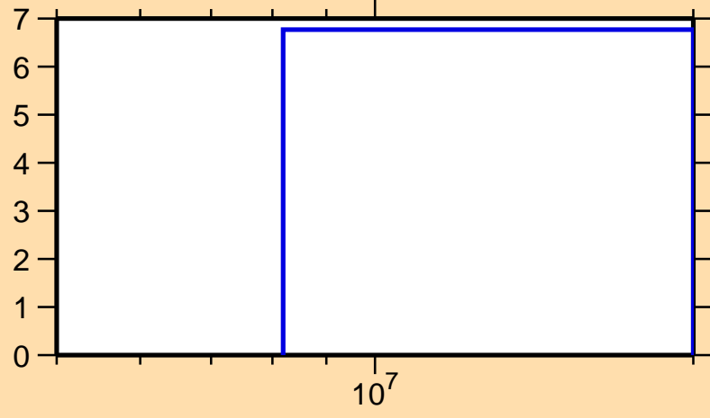
\Delta\sigma/\sigma vs. E for ^{114}\text{Pd}(n,el.)
