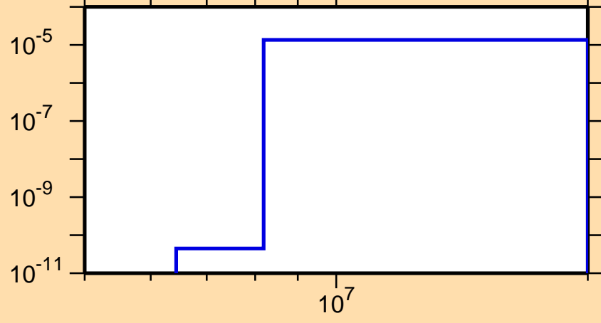
\sigma vs. E for ^{114}\text{Pd}(n,\alpha)
