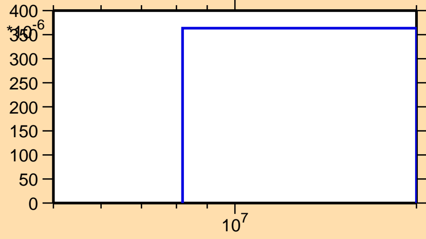
\sigma vs. E for ^{114}\text{Pd}(n,p)
