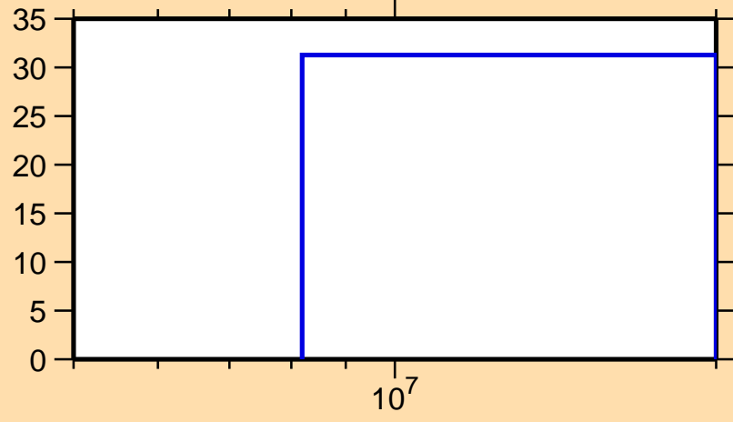
\Delta\sigma/\sigma vs. E for ^{114}\text{Pd}(n,ncont.)
