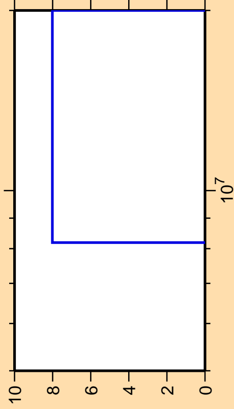
\Delta\sigma/\sigma vs. E for ^{114}\text{Pd}(n,\text{nt})
