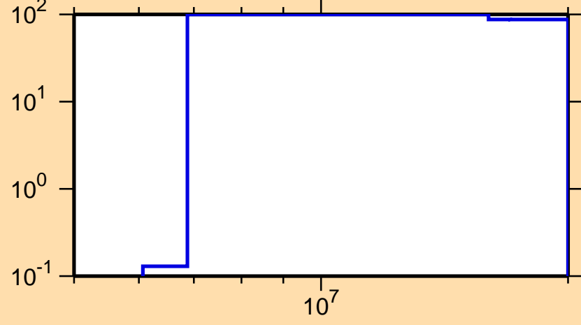
\Delta\sigma/\sigma vs. E for ^{115}\text{Pd}(n,p)
