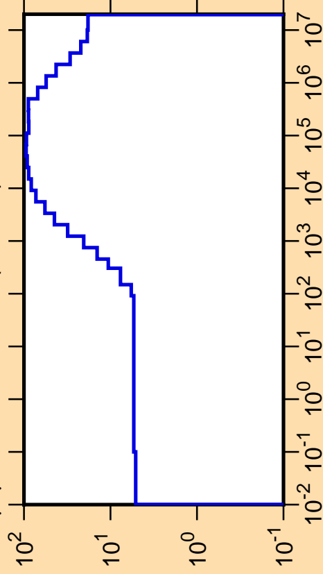
\Delta\mu/\mu vs. E for ^{115}\text{Pd}(\text{mt251})
