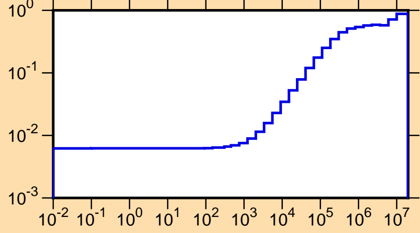
\mu vs. E for ^{115}\text{Pd}(\text{mt251})
