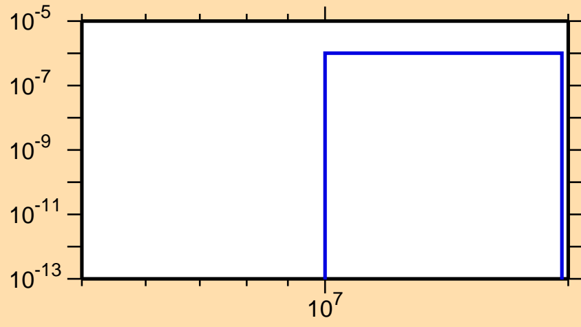
\sigma vs. E for ^{115}\text{Pd}(n,n\alpha)
