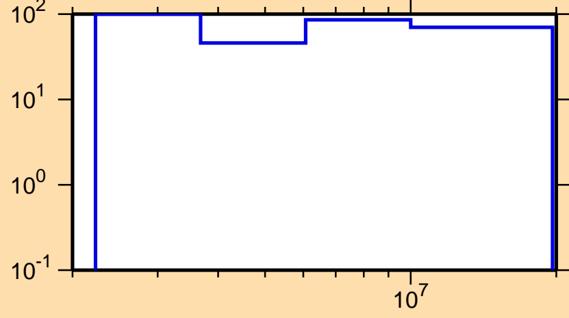
\Delta\sigma/\sigma vs. E for ^{115}\text{Pd}(n,n\text{cont.})
