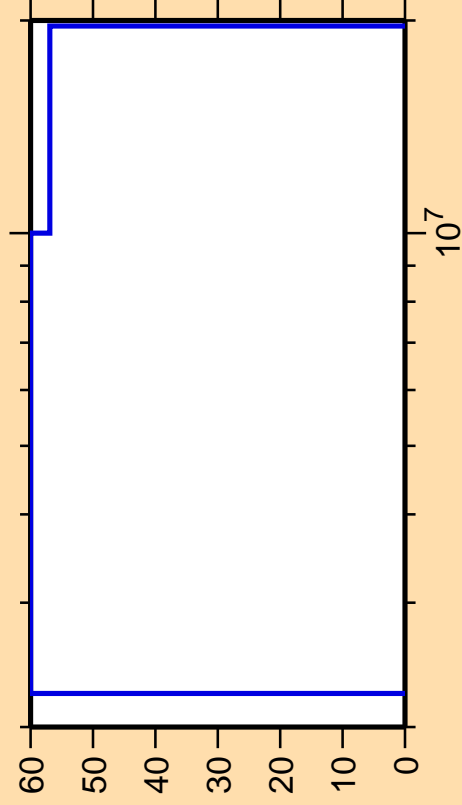
\Delta\sigma/\sigma vs. E for ^{115}\text{Pd}(n,\gamma)
