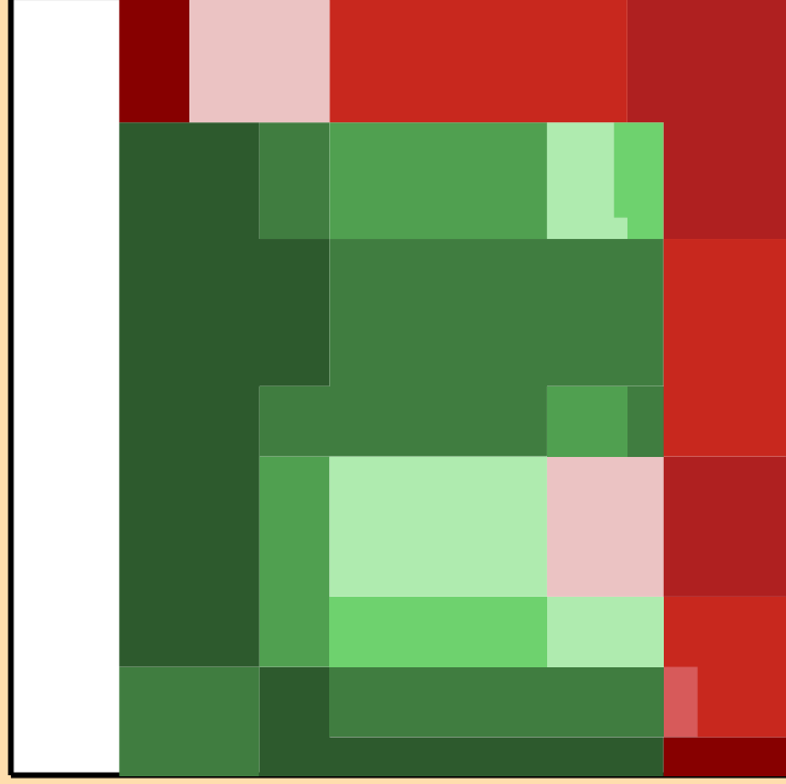
\Delta\sigma/\sigma vs. E for ^{115}\text{Pd}(n,p)
