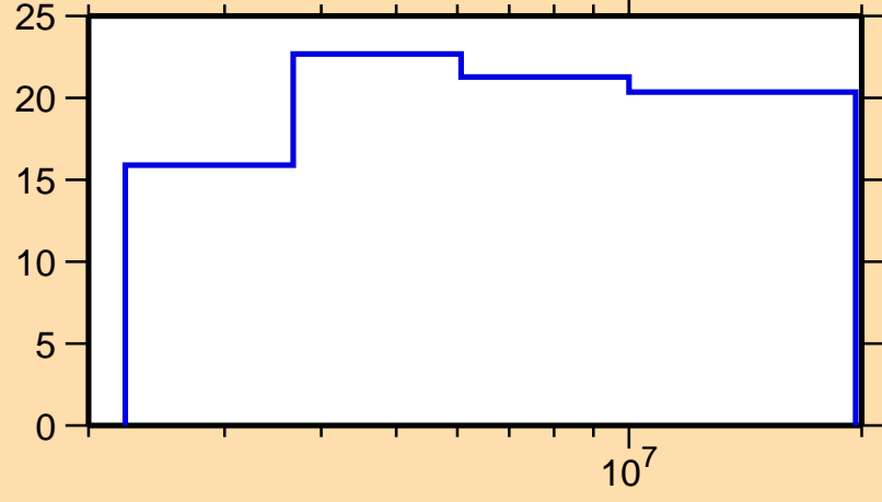
\Delta\sigma/\sigma vs. E for ^{115}\text{Pd}(n,n\text{nonel.})
