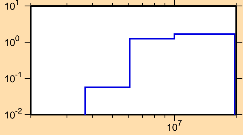
\sigma vs. E for ^{115}\text{Pd}(n,2n)
