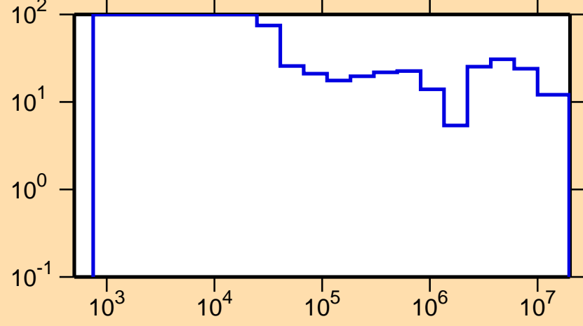
\Delta\sigma/\sigma vs. E for ^{115}\text{Pd}(n,\text{tot.})
