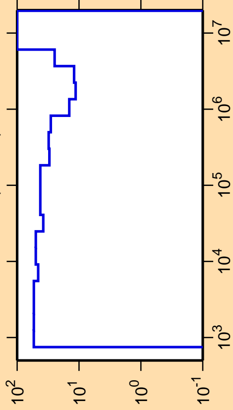
\Delta\sigma/\sigma vs. E for ^{115}\text{Pd}(n,\text{inel.})
