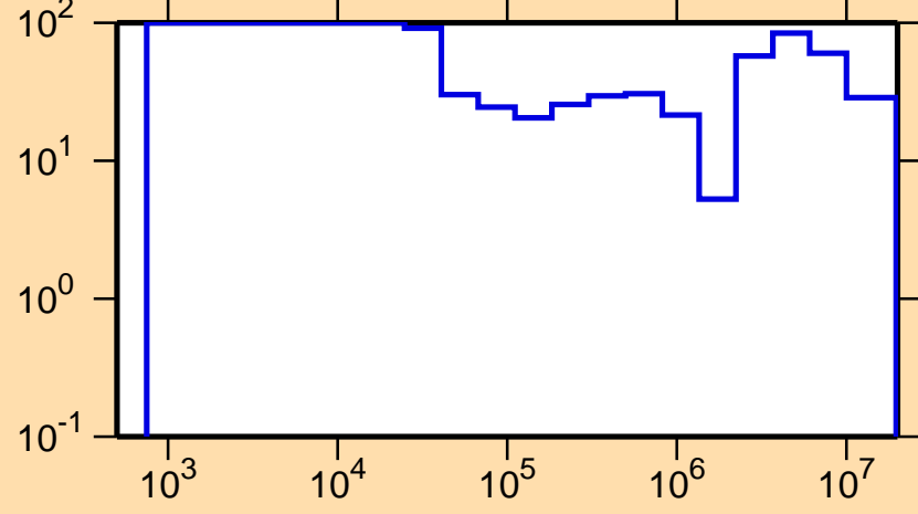
\Delta\sigma/\sigma vs. E for ^{115}\text{Pd}(n,\text{el.})
