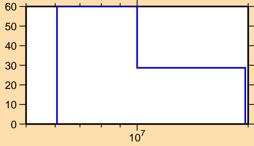
\Delta\sigma/\sigma vs. E for ^{115}\text{Pd}(n,el.)
