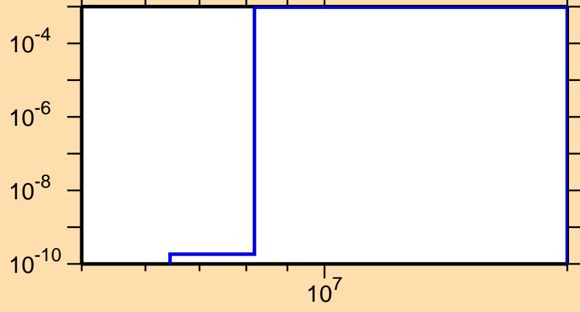
\sigma vs. E for ^{115}\text{Pd}(n,p)
