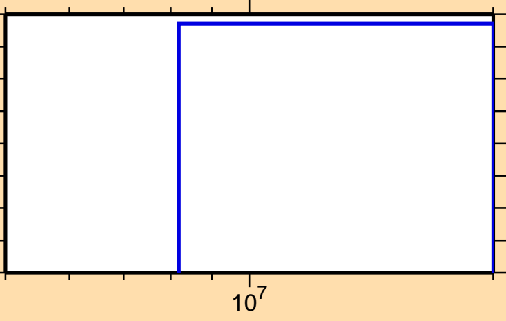
\sigma vs. E for ^{115}\text{Pd}(n,np)
