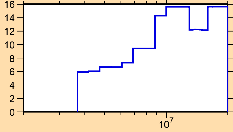
\Delta\sigma/\sigma vs. E for ^{117}\text{Pd}(n,n\text{nonel.})
