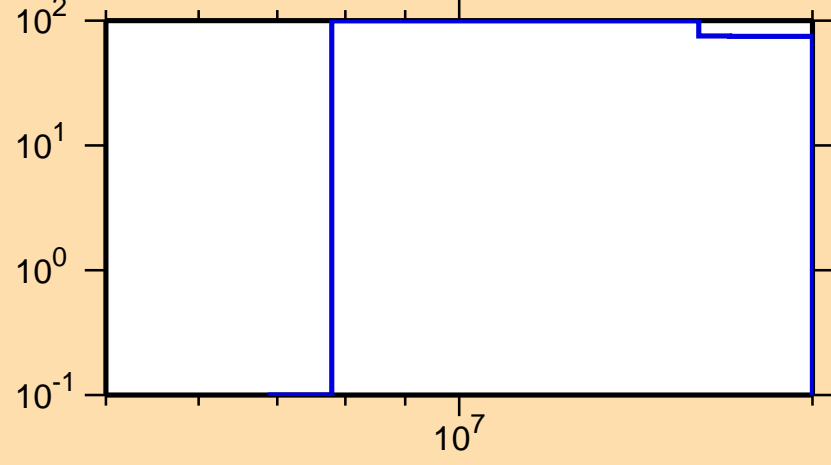
\Delta\sigma/\sigma vs. E for ^{117}\text{Pd}(n,p)
