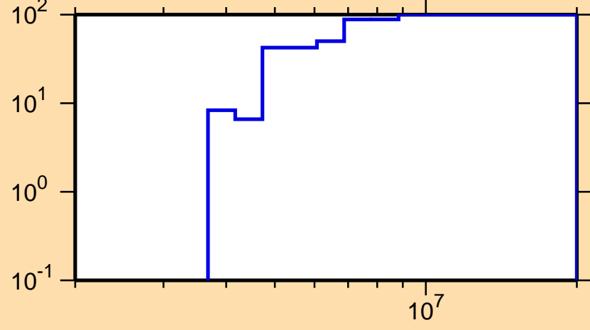
\Delta\sigma/\sigma vs. E for ^{117}\text{Pd}(n,\text{inel.})
