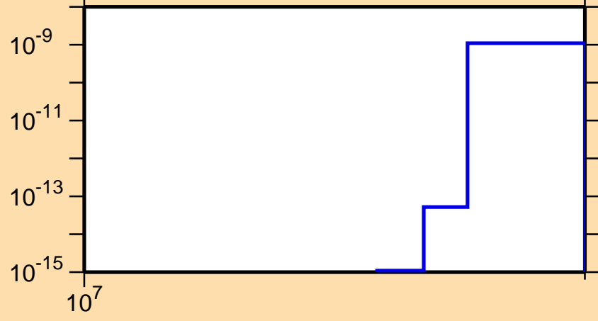
\sigma vs. E for ^{117}\text{Pd}(n,nt)
