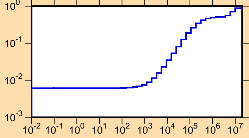
\mu vs. E for ^{117}\text{Pd}(\text{mt251})
