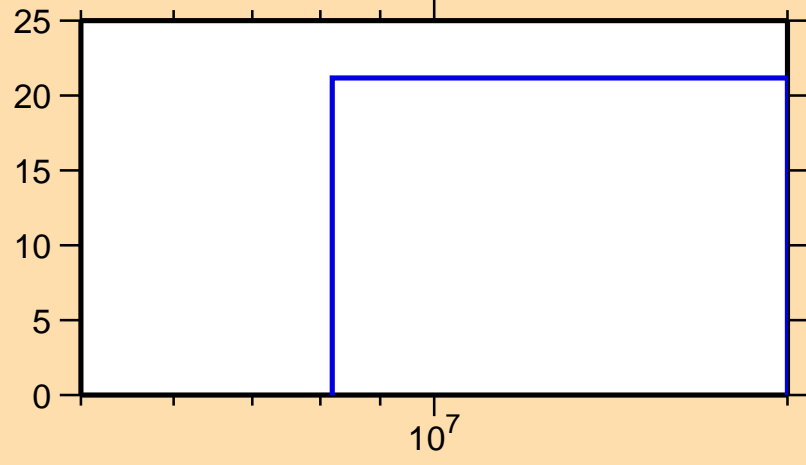
\Delta\sigma/\sigma vs. E for ^{118}\text{Pd}(n,el.)
