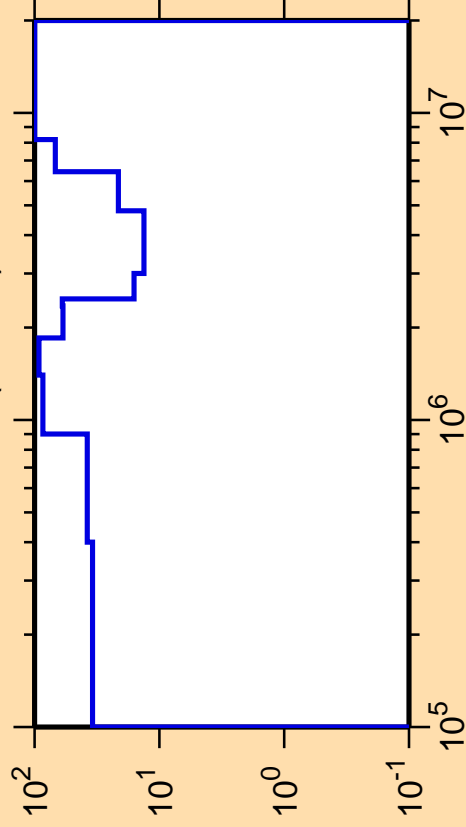
\Delta\sigma/\sigma vs. E for ^{118}\text{Pd}(n,\text{inel.})
