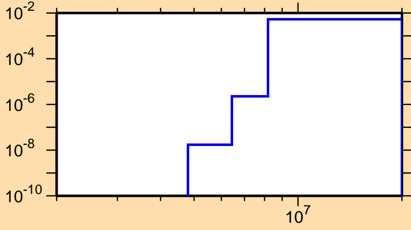
\sigma vs. E for ^{195}\text{Po}(n,d)
