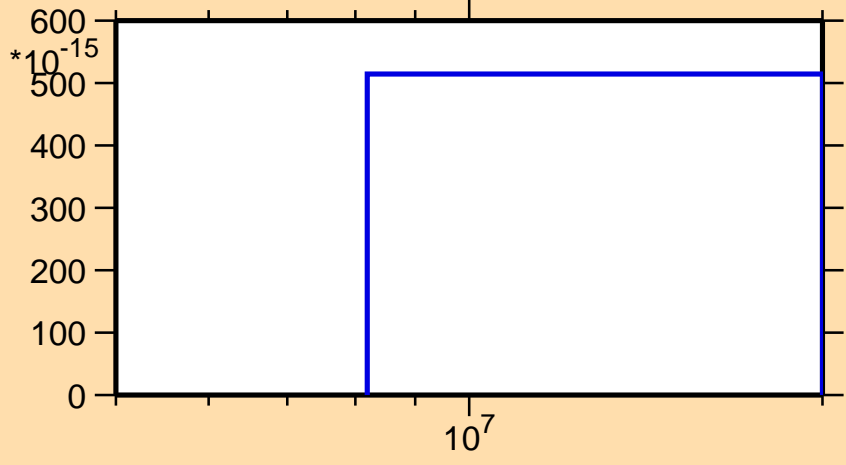
\sigma vs. E for ^{195}\text{Po}(n,\text{nt})
