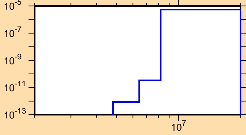
\sigma vs. E for ^{195}\text{Po}(n,\text{He3})
