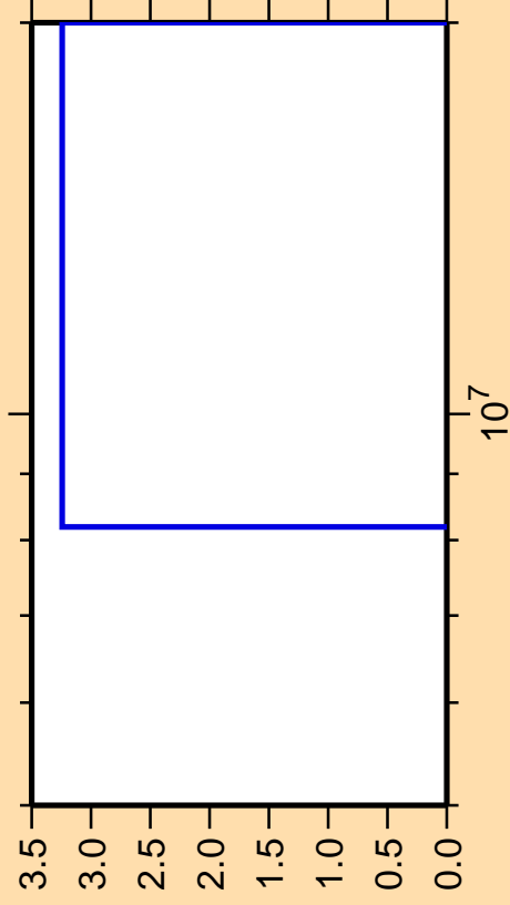
\Delta\sigma/\sigma vs. E for ^{195}\text{Po}(n,\text{nt})
