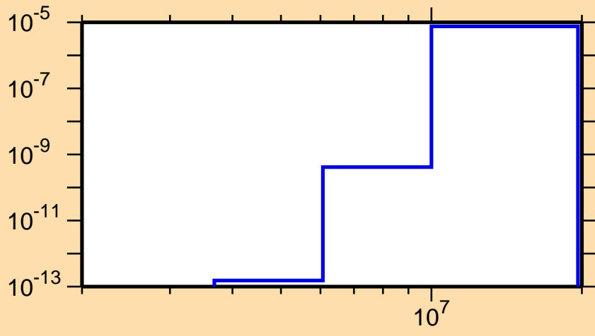
\sigma vs. E for ^{195}\text{Po}(n,\text{He3})
