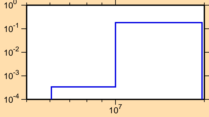
\sigma vs. E for ^{195}\text{Po}(n,2n)
