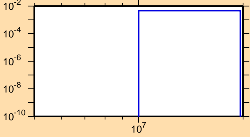
\sigma vs. E for ^{195}\text{Po}(n,2n\alpha)
