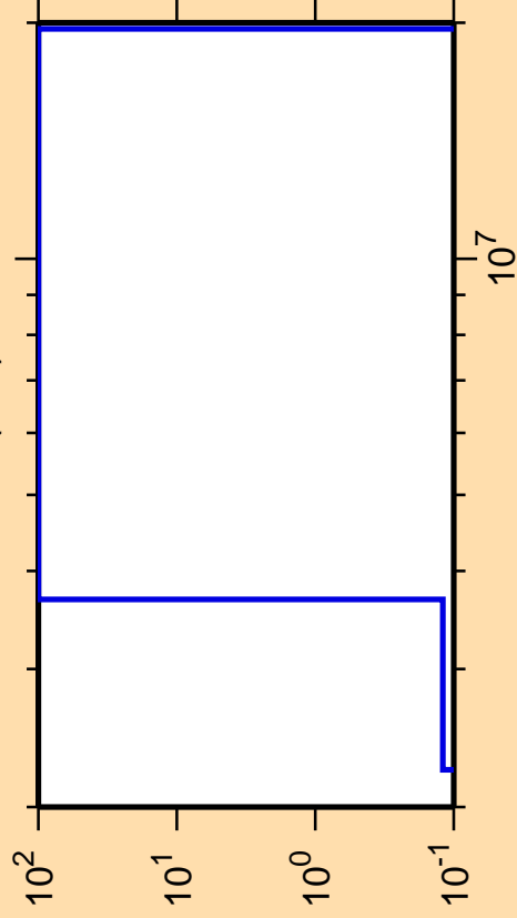
\Delta\sigma/\sigma vs. E for ^{195}\text{Po}(n,d)
