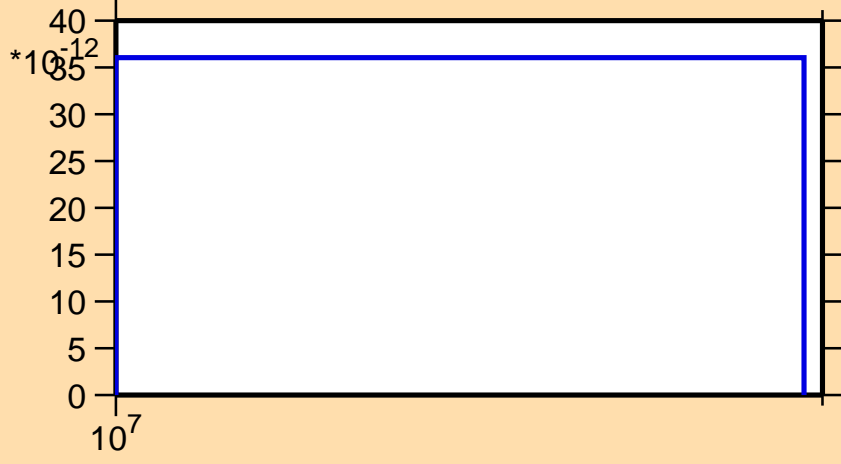
\sigma vs. E for ^{195}\text{Po} (mt 34)
