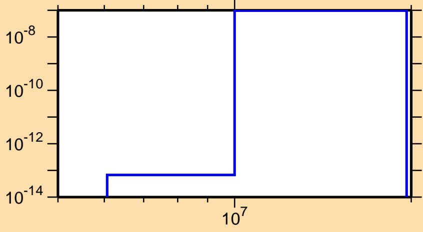
\sigma vs. E for ^{195}\text{Po}(\text{mt } 45)
