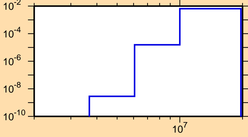
\sigma vs. E for ^{195}\text{Po}(n,d)
