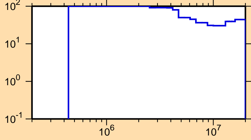
\Delta\sigma/\sigma vs. E for ^{196}\text{Po}(n,\text{inel.})
