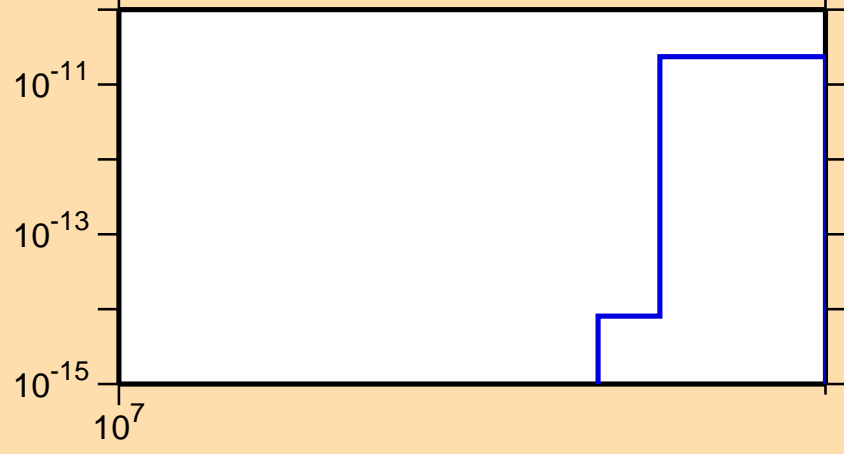
\sigma vs. E for ^{196}\text{Po}(n,nt)
