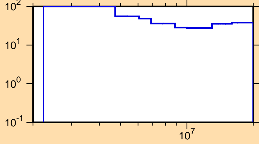
\Delta\sigma/\sigma vs. E for ^{196}\text{Po}(n,n\text{cont.})
