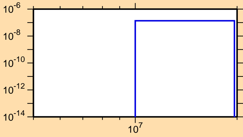
\sigma vs. E for ^{196}\text{Po}(n,2n\alpha)
