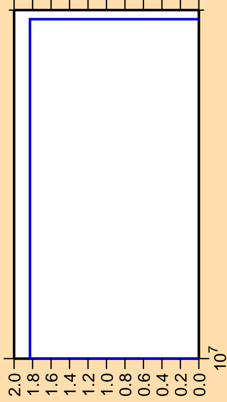
\Delta\sigma/\sigma vs. E for ^{196}\text{Po} (mt 34)
