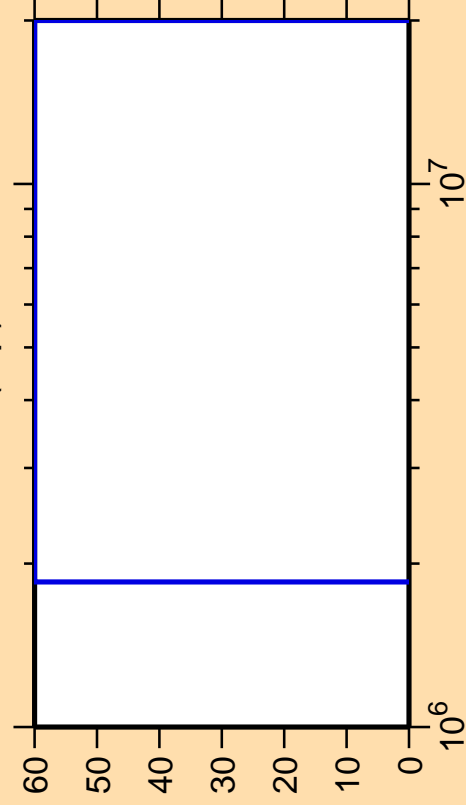
\Delta\sigma/\sigma vs. E for ^{196}\text{Po}(n,p)
