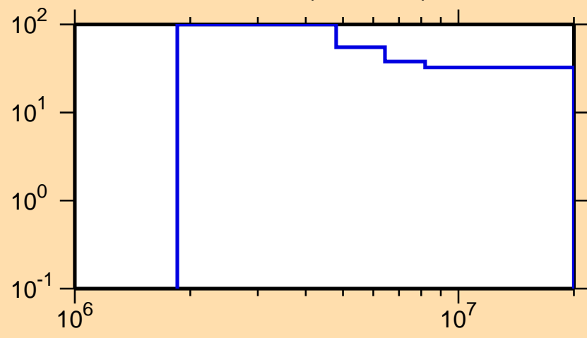
\Delta\sigma/\sigma vs. E for ^{196}\text{Po}(n,n\text{cont.})
