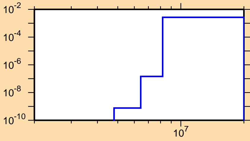
\sigma vs. E for ^{196}\text{Po}(n,d)
