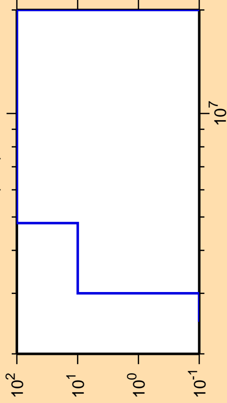
\Delta\sigma/\sigma vs. E for ^{196}\text{Po}(n,d)
