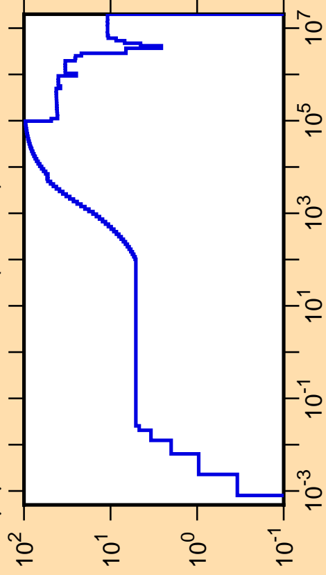
\Delta\mu/\mu vs. E for ^{197}\text{Po}(\text{mt251})
