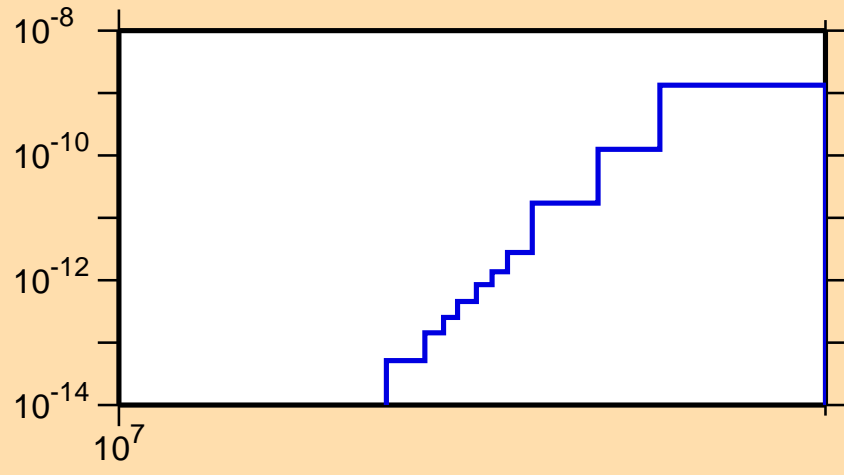
\sigma vs. E for ^{197}\text{Po}(\text{mt } 34)
