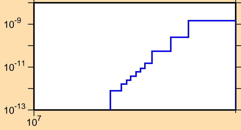
\sigma vs. E for ^{197}\text{Po}(\text{mt117})
