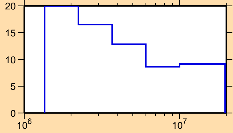
\Delta\sigma/\sigma vs. E for ^{197}\text{Po}(n,n\text{nonel.})
