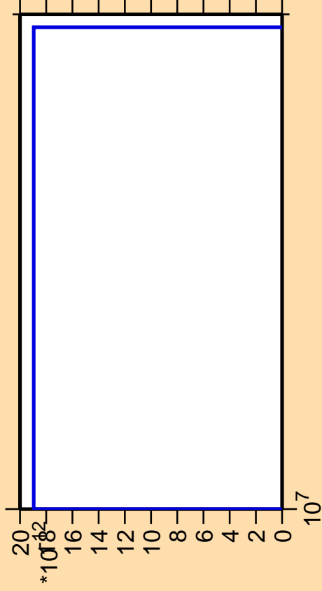
\Delta\sigma/\sigma vs. E for ^{197}\text{Po} (mt 11)
